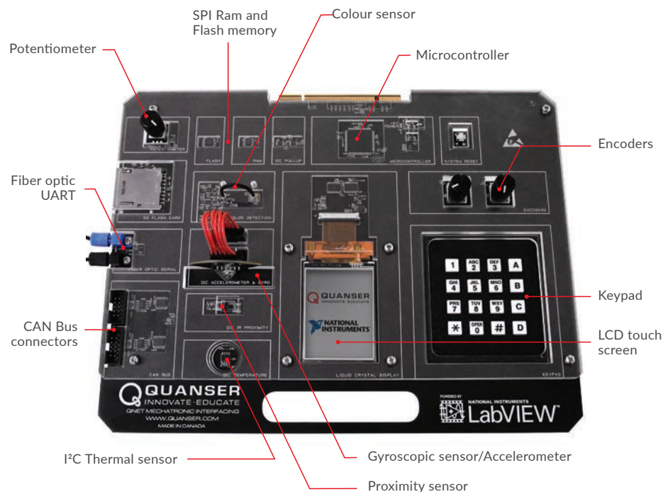
Mechatronic Interfacing Board
